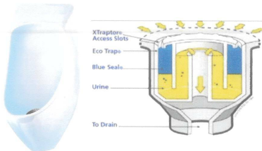
Waterless Urinal
